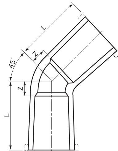
呼び径 75~100mm
